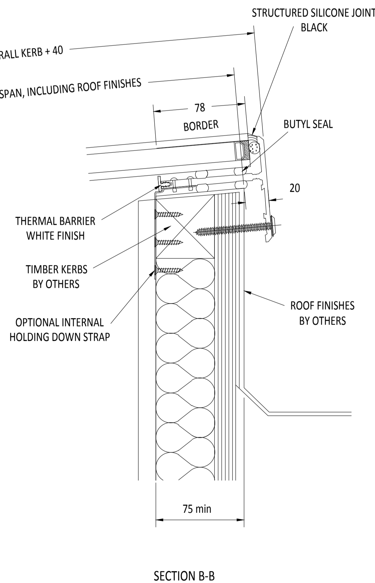
SECTION B-B
