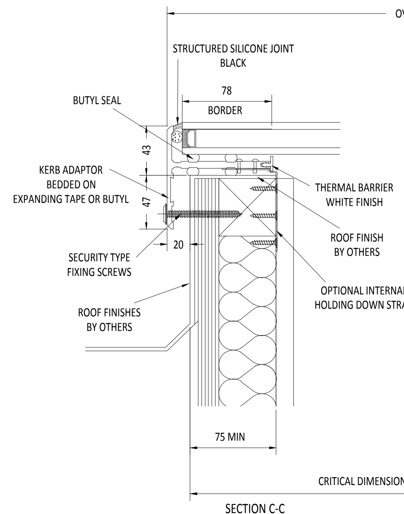
SECTION C-C
